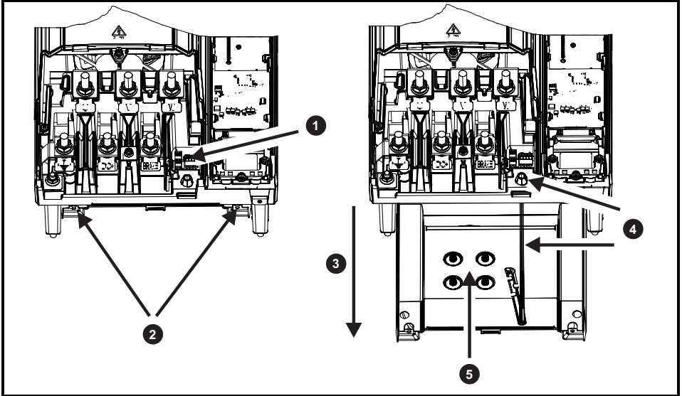
Figure 3-13 Heatsink fan replacement
