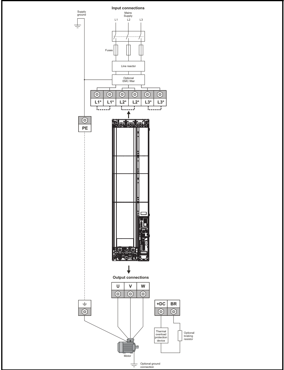
Figure 4-1 Power connections
